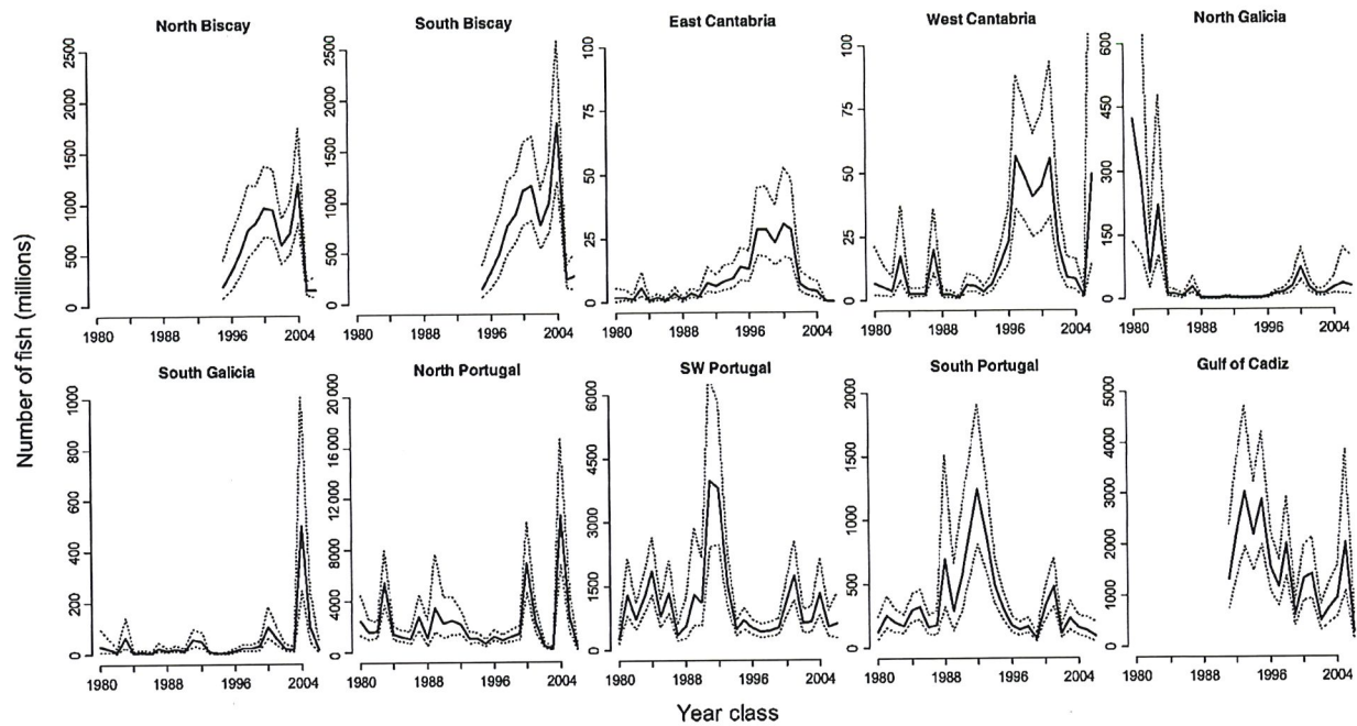
Figure 6. Temporal variation in sardine recruitment (at age 1, solid line) by area in acoustic surveys, predicted (anti-logged) by year-class models assuming the same (French surveys, Model 5) or variable year-class strength by area (Models 4 and 6 for Portuguese and Spanish surveys, respectively). Dotted lines shows predicted values \pm 1 s.e. Note the differences in the y-axis scales.
