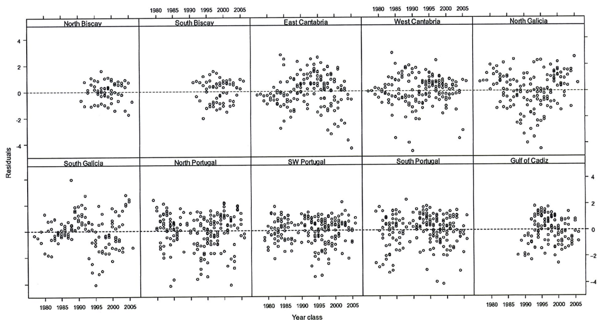
Figure 4. Residuals by year class for final YCC models fitted to French (Model 5), Spanish (Model 5), and Portuguese (Model 3) acoustic surveys.
